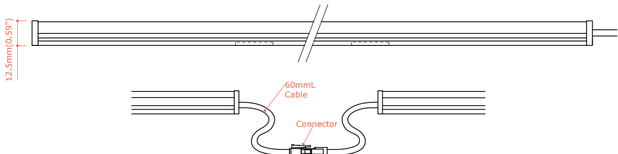
FRONT VIEW
