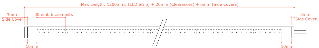
TOP VIEW
