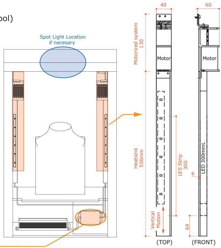
(Installation example)
