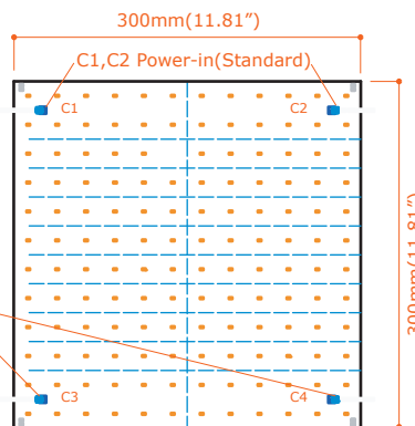
Standard Configuration CL300
