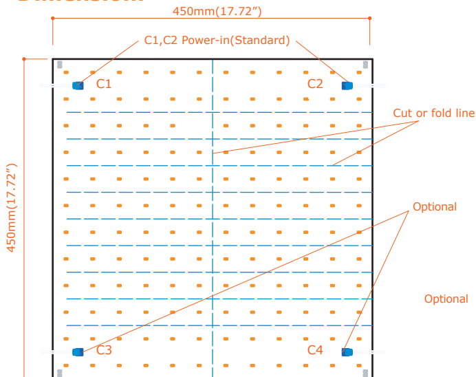
Standard Configuration CL450
